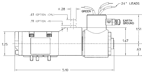
Figure 4. Pneumatic Solenoid
